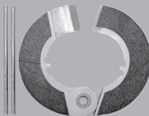
MID-AMERICA CLUTCH HINGED CLUTCH BRAKE .375 HB200
